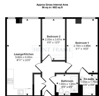
Floorplan
